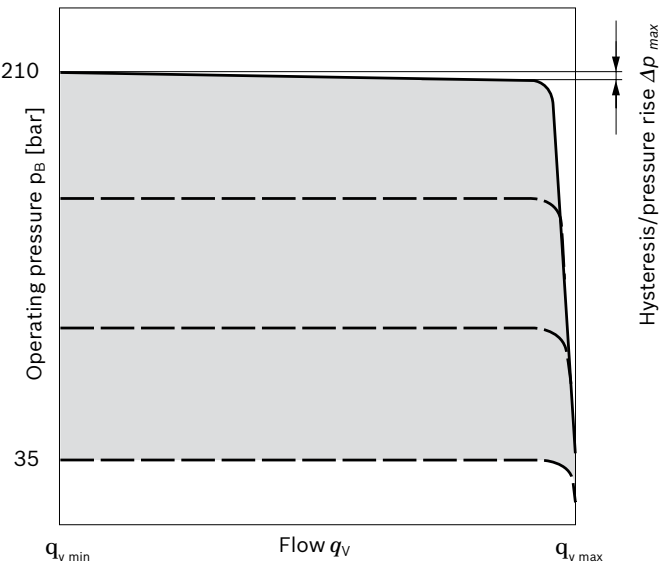
Characteristic curve valid at n_1 = 1500 \text{ rpm} and \theta_{\text{fluid}} = 50 \text{ }^\circ\text{C} .
